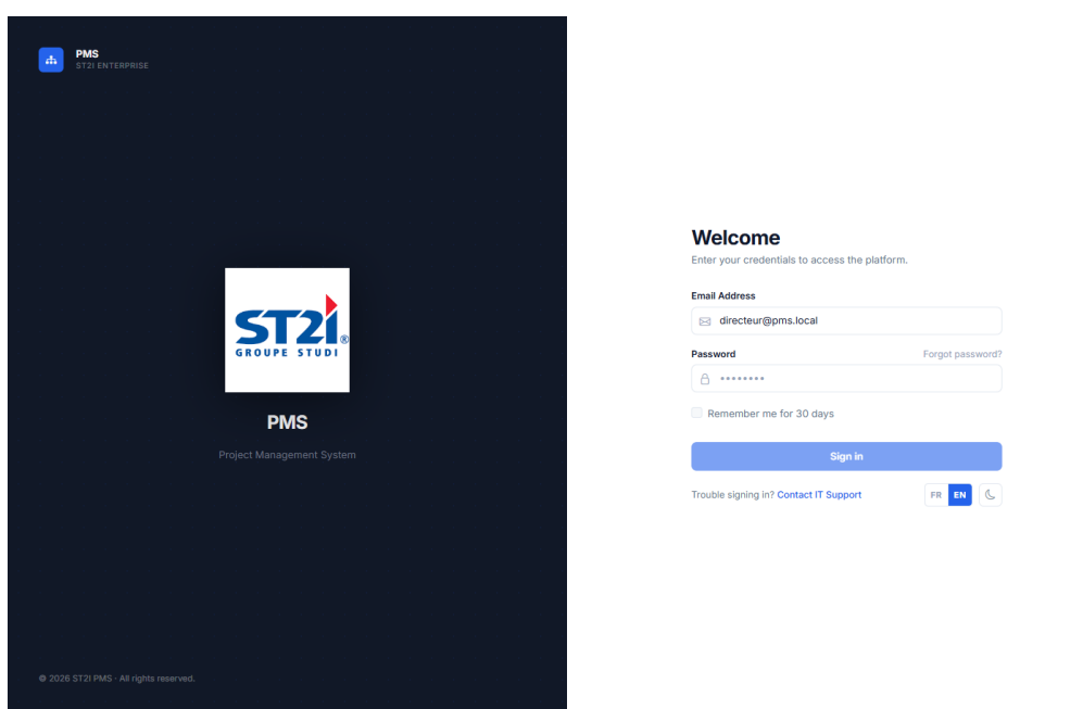
Figure 4.12: Login interface
